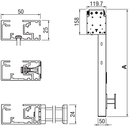
VA3100 Hide 1-piece guide rail VA110
