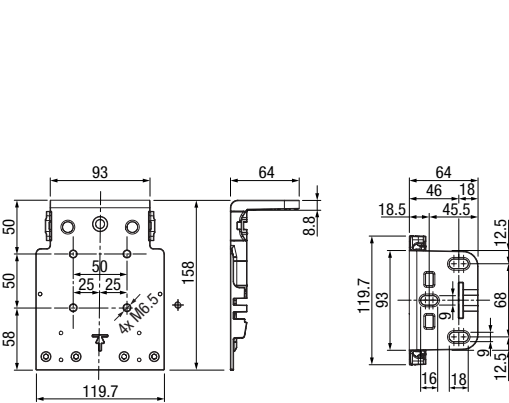
VA3100 Hide Ceiling / floating bracket VA310
