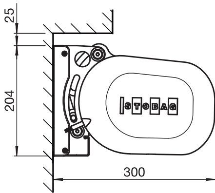
BX8000 Wandmontage
