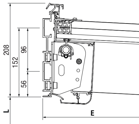
GP4100 Raccordement mural
