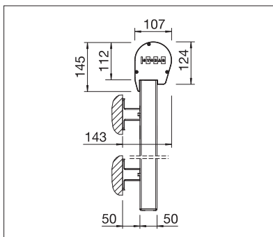
Wall fixing with round box and guide profile
