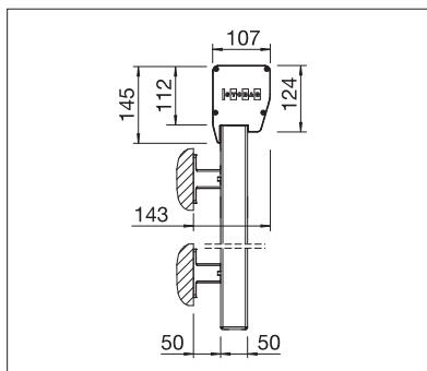
Wall fixing with square box and guide profile
